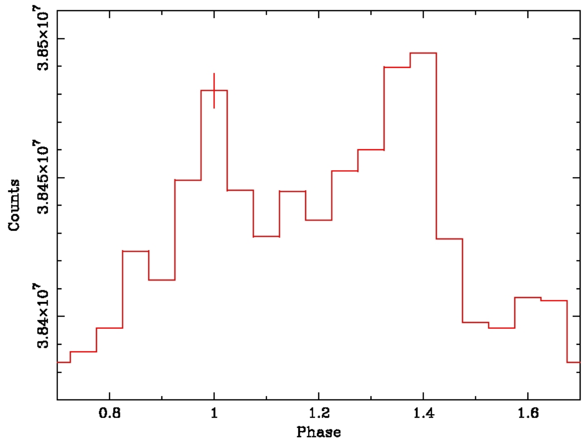
Folded lightcurve (260-364 keV)
