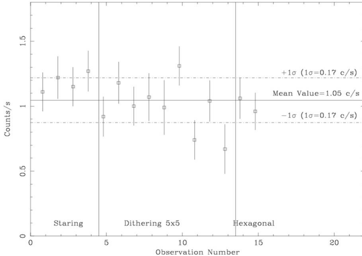
Crab on-axis (Rev. 39-45): Energy Band 3 (336-448 keV)
