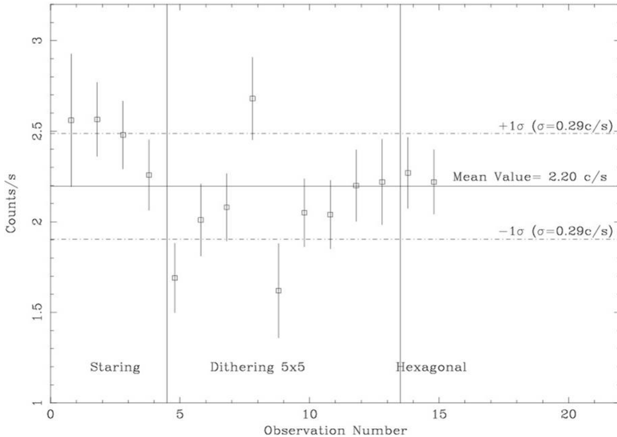
Crab on-axis (Rev. 39-45): Energy Band 2 (252-336 keV)
