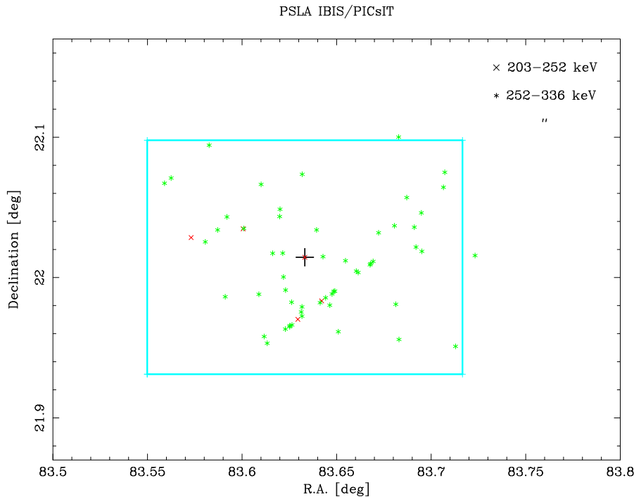
Figure 6: Sky coordinate reconstruction of the Crab position obtained with the ScW detections with SNR > 3\sigma (Exposure 5 ks) in the energy band 252 – 336 keV (*) and 203 – 252 keV (x). The catalog position of the Crab is shown at the centre of the figure and indicated with +. The surrounding square represents the pixel of PICsIT with 10' size.
