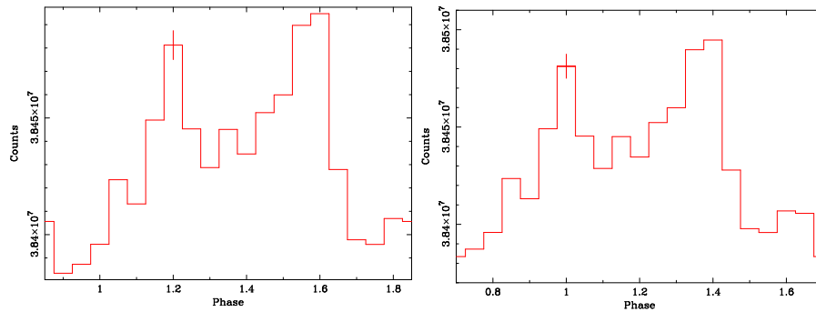
Figure 7: ( left ) Crab observation during the rev 40 – 41 (spectral timing, 1 ms time resolution). Uncorrected folded lightcurve in the energy band 260 – 364 keV. ( right ) The same as above, but corrected manually for the residual shift in phase of 0.2. Courtesy T. Mineo.
