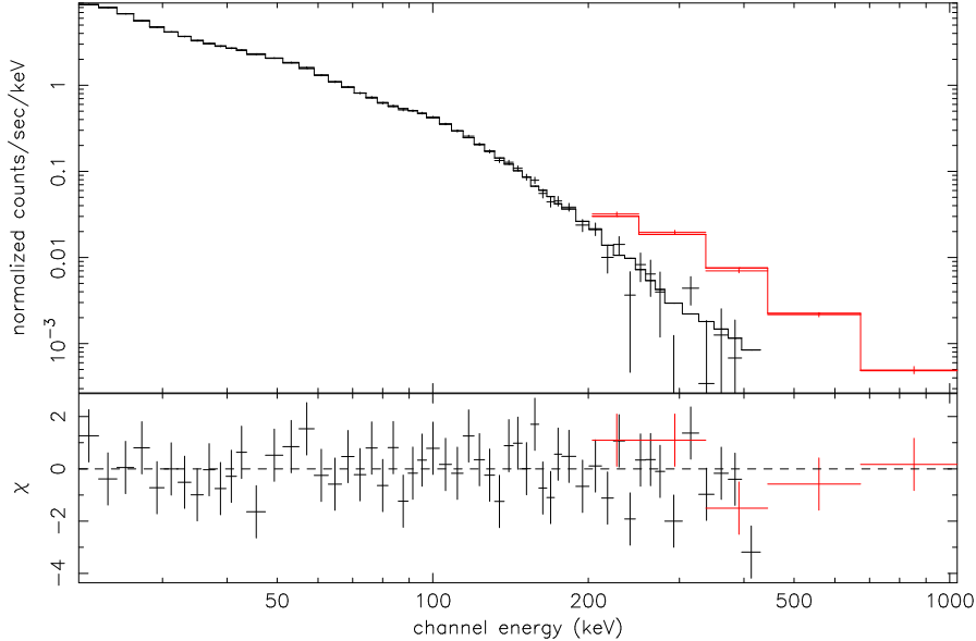
Figure 6: IBIS (ISGRI+PICsIT) spectrum of the Crab. Data of ISGRI are from rev. 102, while data of PICsIT are from the standard mode Scw in the revs. 39 – 45 (courtesy L. Natalucci).
