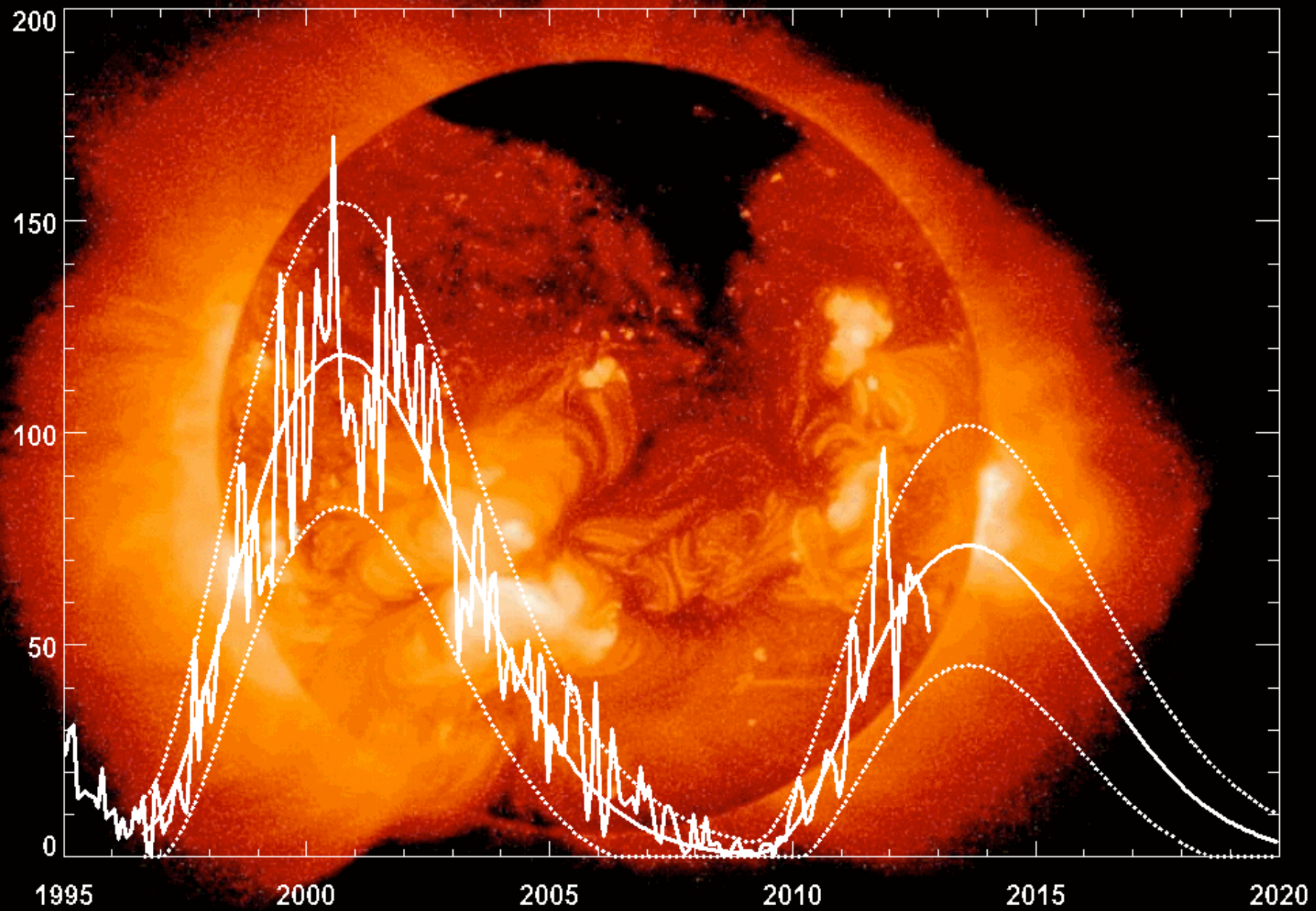
Cycle 24 Sunspot Number Prediction (November 2012)
